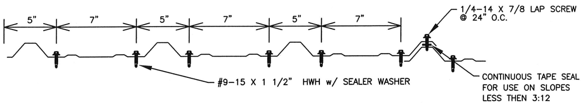
FASTENER PATTERN AT PANEL ENDS
