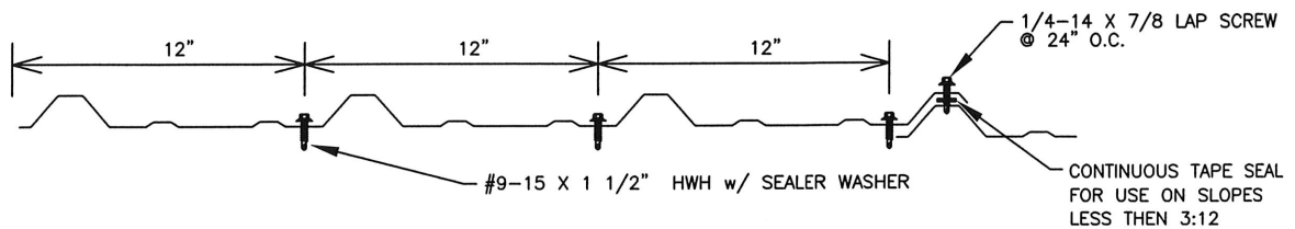
TYPICAL FASTENER PATTERN
